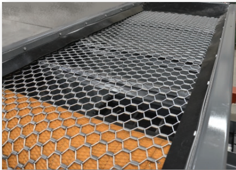
60" Stick Remover and Sizer (shown with trash conveyor)
